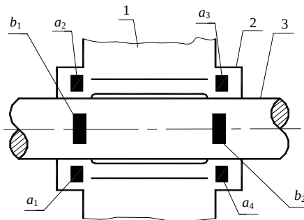
1 - 轴承座; 2 - 轴瓦; 3 - 轴
